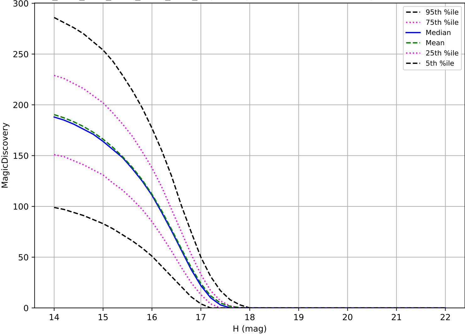
ddf_acor_sf20_lsf30_lsr50_v3.4_10yrs: Trojan 6 detections in 60 nights detection loss
