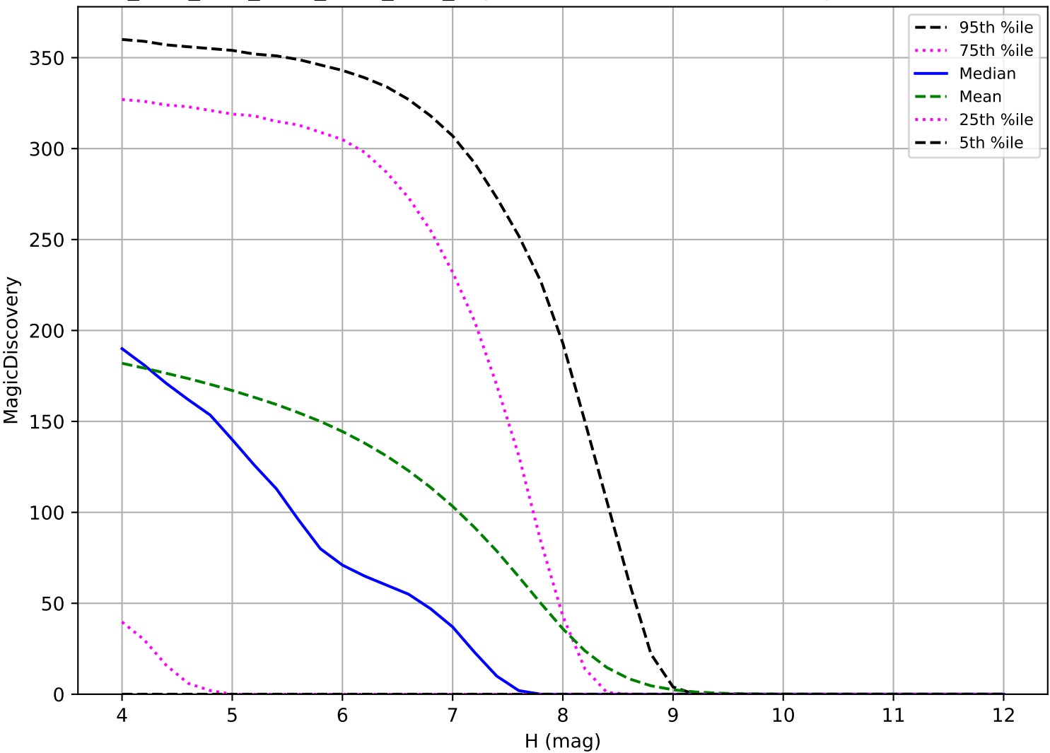
ddf_acor_sf20_lsf30_lsr50_v3.4_10yrs: TNO 6 detections in 60 nights detection loss
