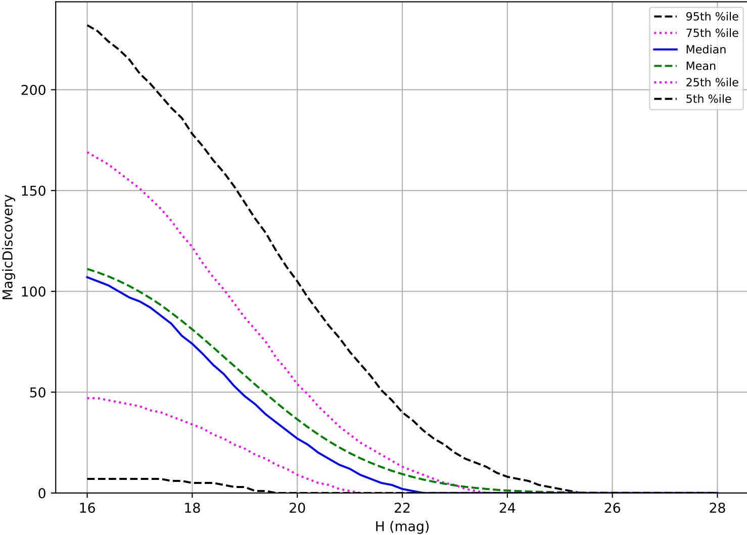
ddf_acor_sf20_lsf30_lsr50_v3.4_10yrs: PHA 6 detections in 60 nights detection loss
