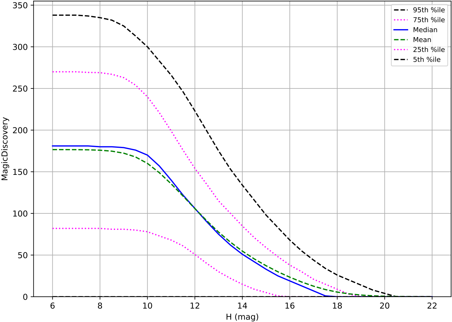
ddf_acor_sf20_lsf30_lsr50_v3.4_10yrs: OCC_r5 6 detections in 60 nights detection loss
