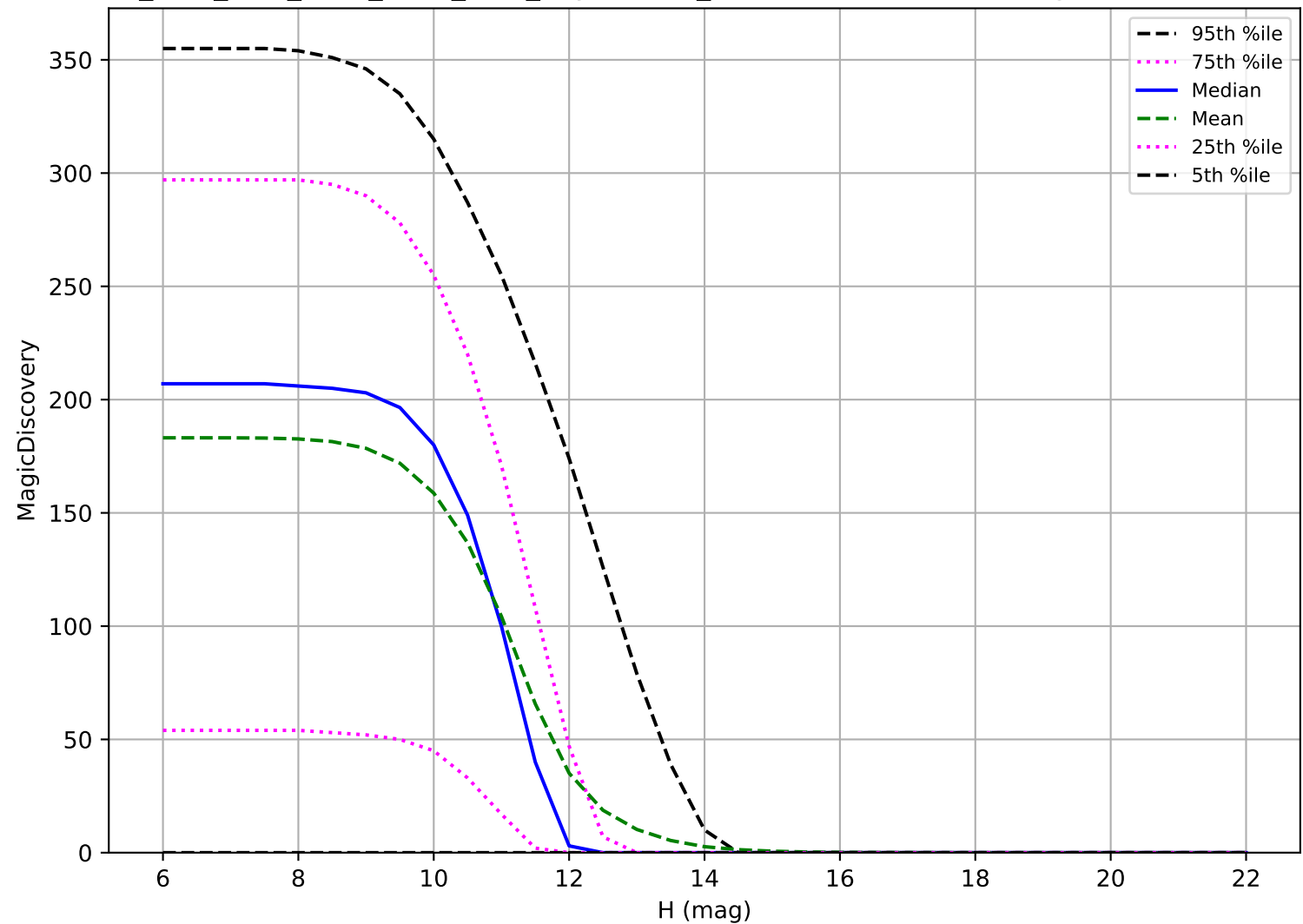
ddf_acor_sf20_lsf30_lsr50_v3.4_10yrs: OCC_r20 6 detections in 60 nights detection loss
