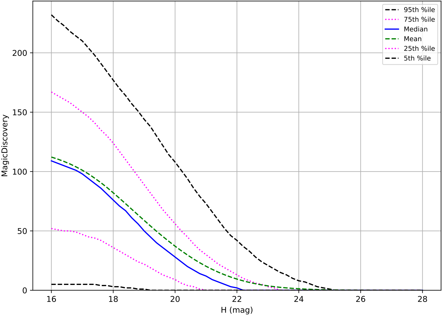
ddf_acor_sf20_lsf30_lsr50_v3.4_10yrs: NEO 6 detections in 60 nights detection loss
