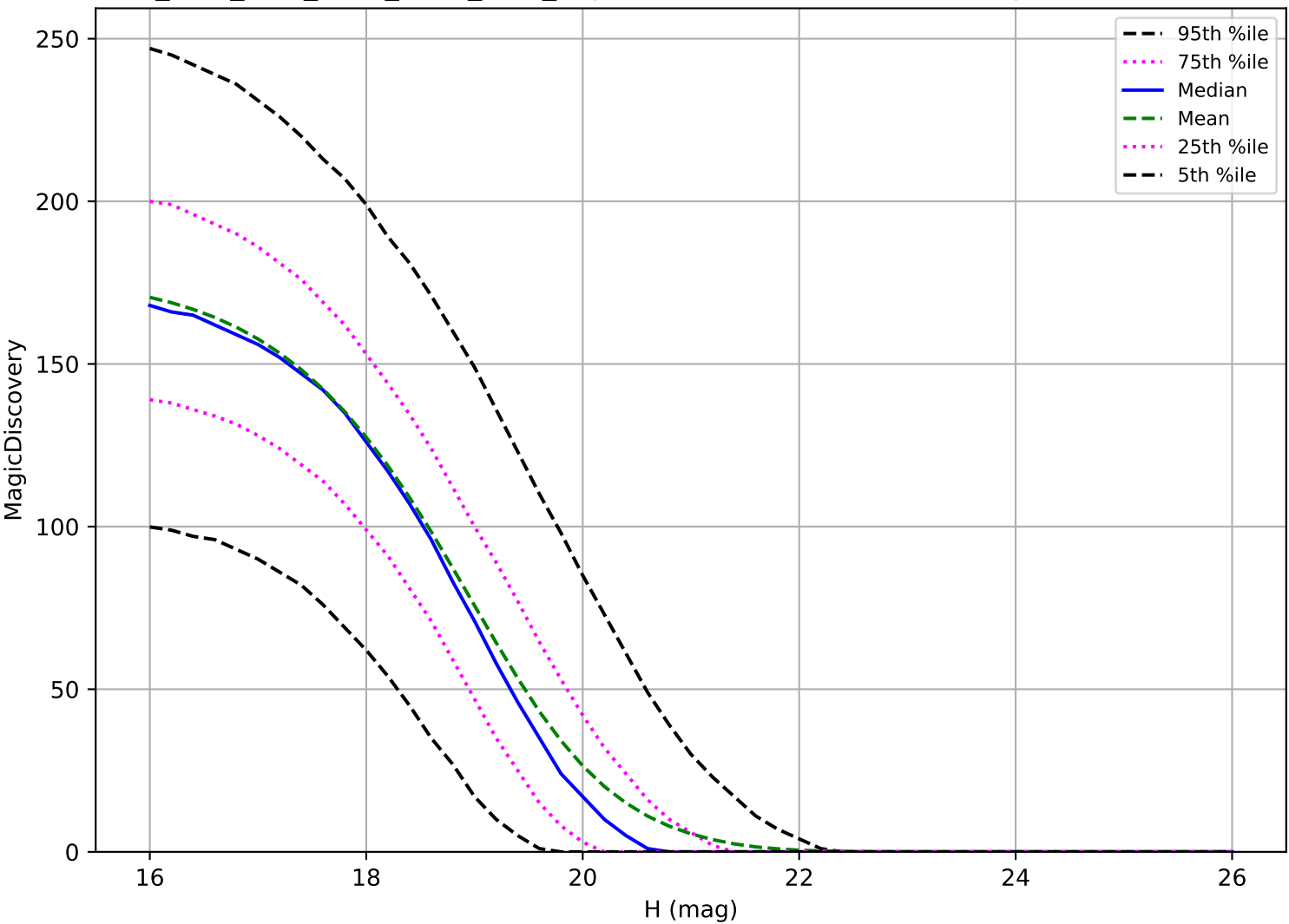
ddf_acor_sf20_lsf30_lsr50_v3.4_10yrs: MBA 6 detections in 60 nights detection loss
