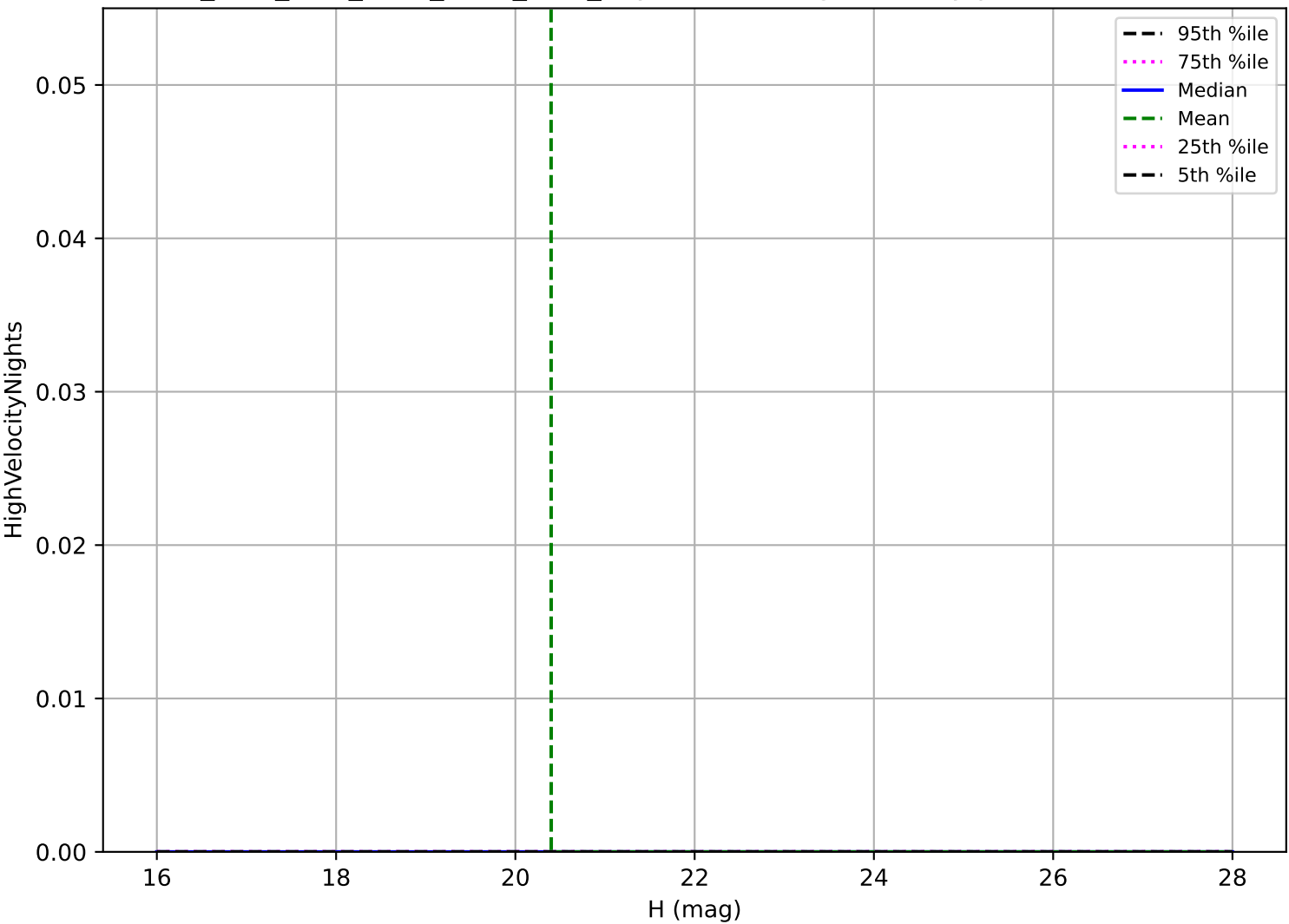
ddf_acor_sf20_lsf30_lsr50_v3.4_10yrs: Vatira High velocity pair detection loss
