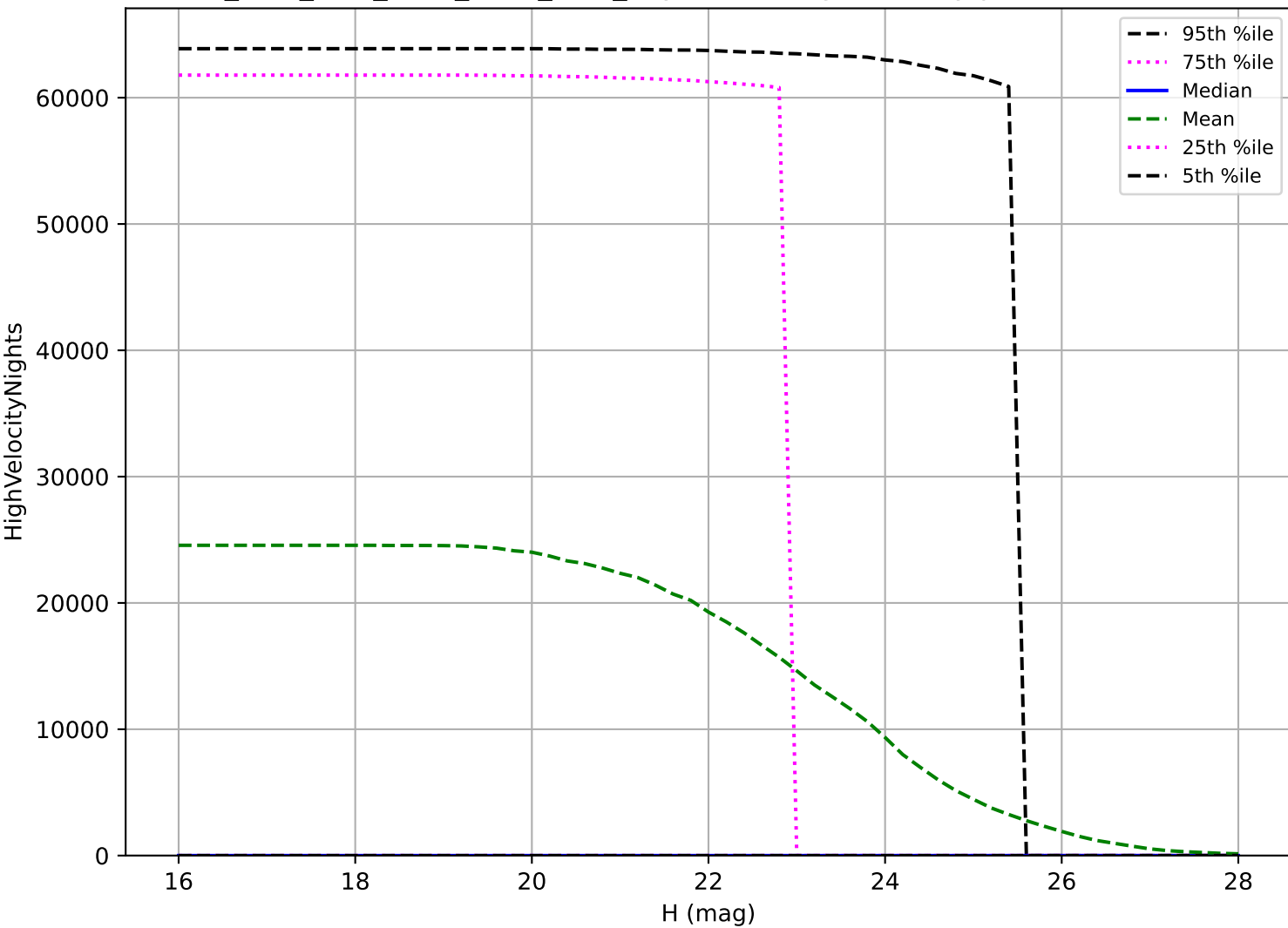
ddf_acor_sf20_lsf30_lsr50_v3.4_10yrs: PHA High velocity pair detection loss
