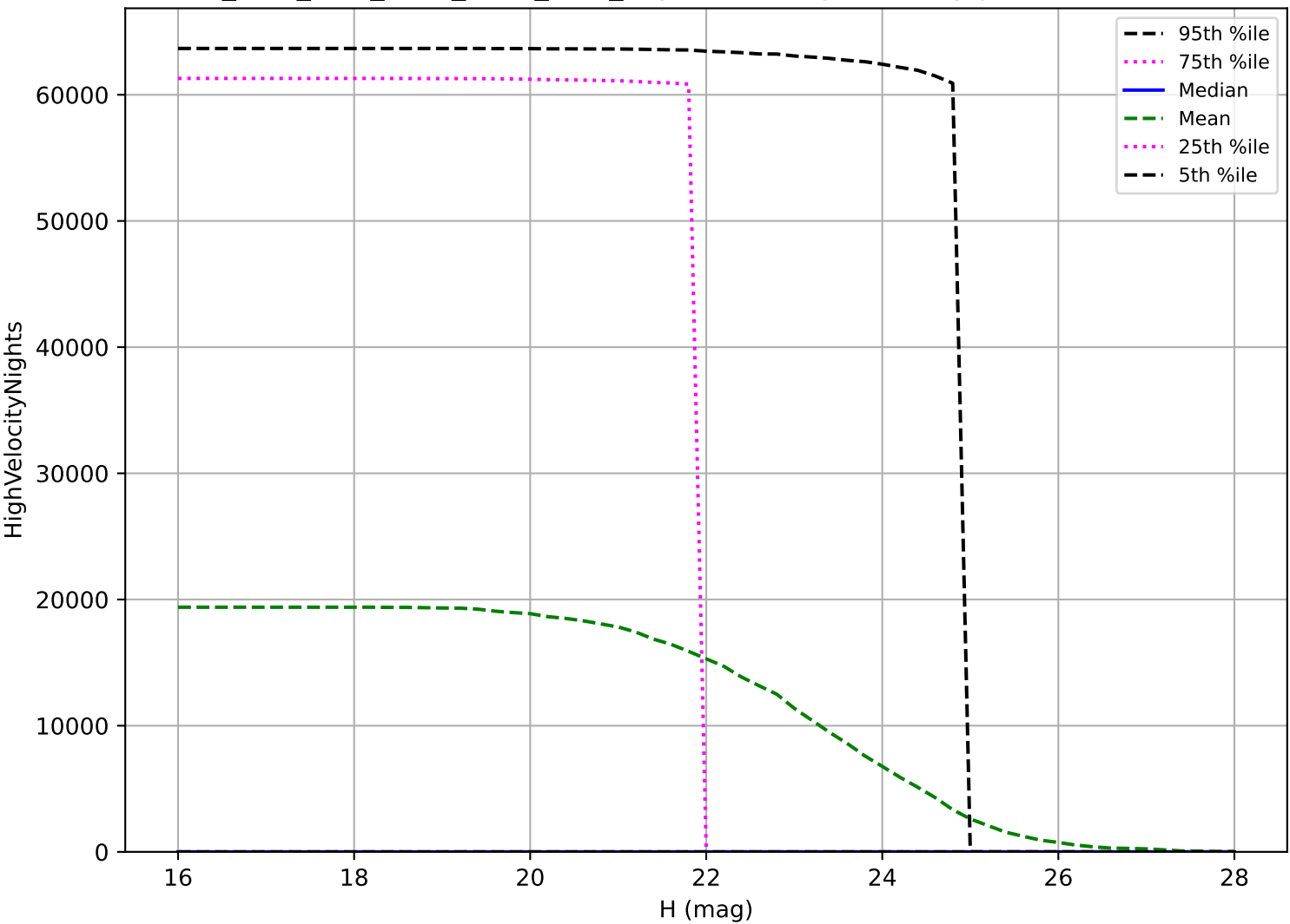
ddf_acor_sf20_lsf30_lsr50_v3.4_10yrs: NEO High velocity pair detection loss
