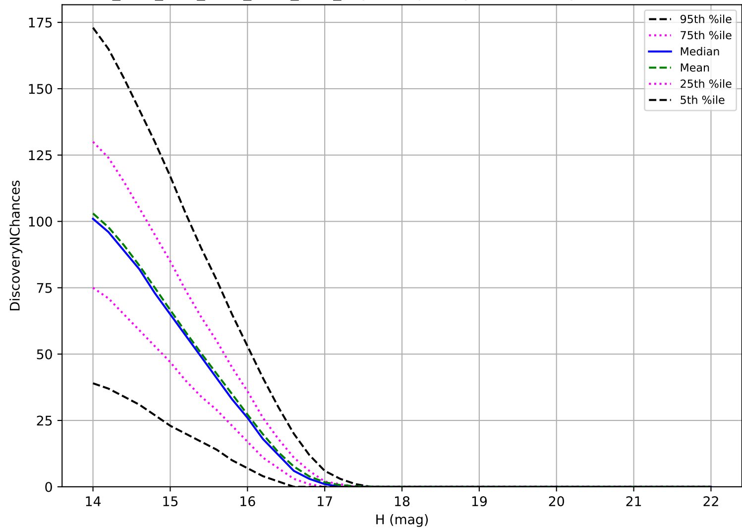
ddf_acor_sf20_lsf30_lsr50_v3.4_10yrs: Trojan 3 pairs in 15 nights detection loss
