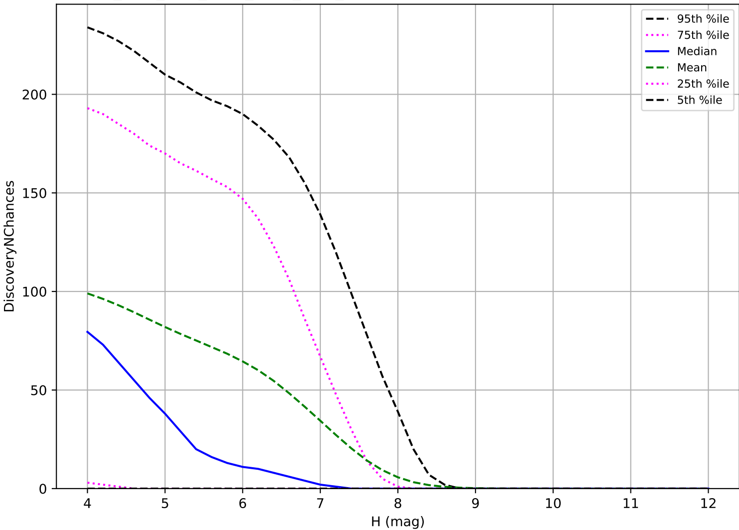
ddf_acor_sf20_lsf30_lsr50_v3.4_10yrs: TNO 3 pairs in 15 nights detection loss
