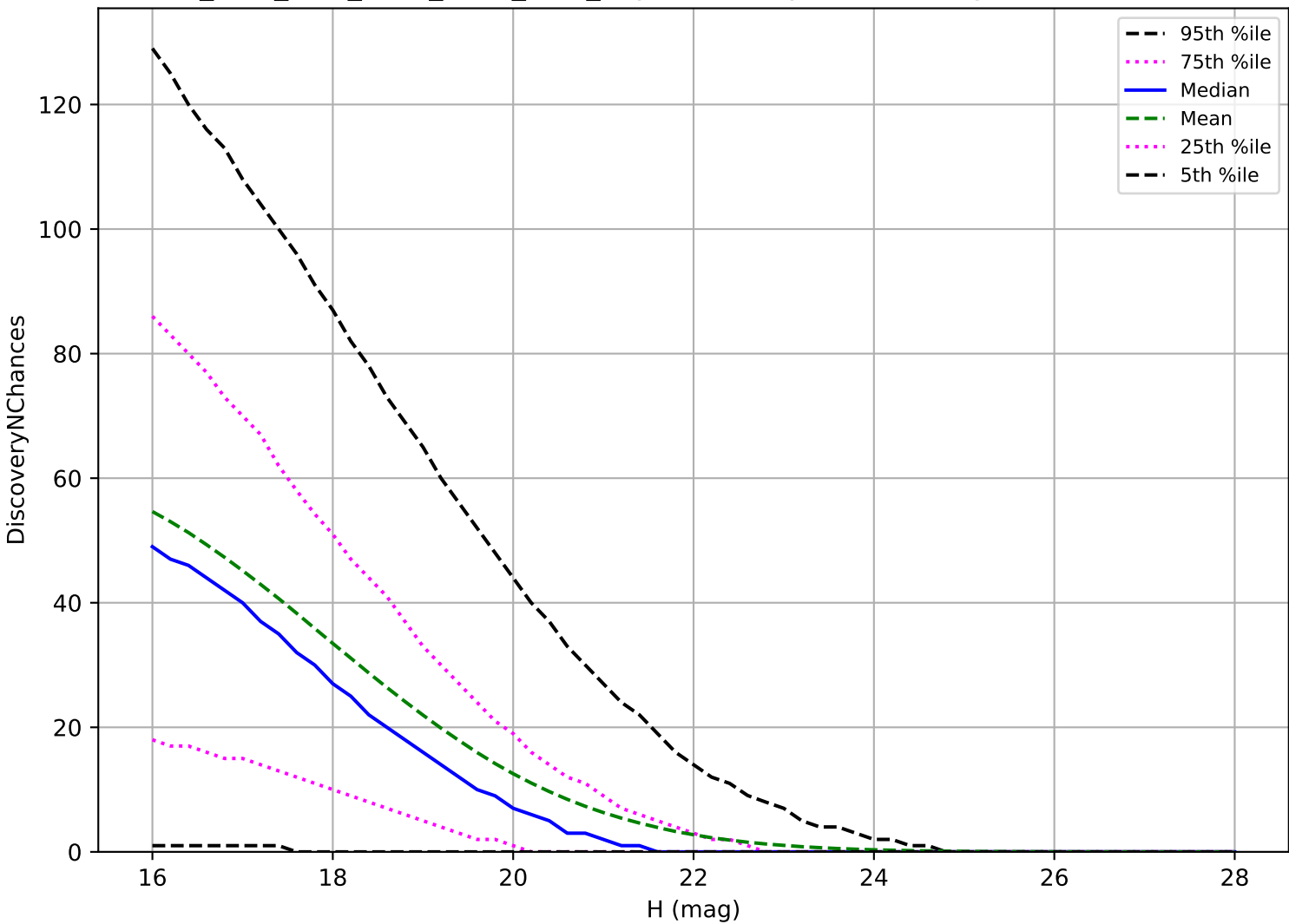
ddf_acor_sf20_lsf30_lsr50_v3.4_10yrs: PHA 3 pairs in 15 nights detection loss
