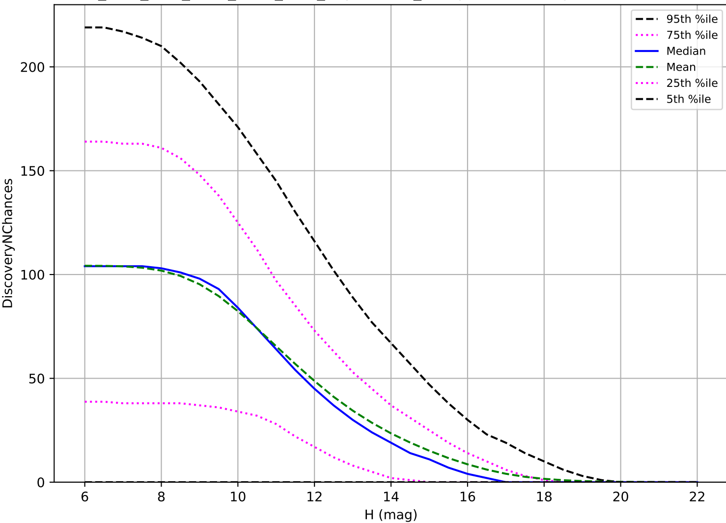
ddf_acor_sf20_lsf30_lsr50_v3.4_10yrs: OCC_r5 3 pairs in 15 nights detection loss
