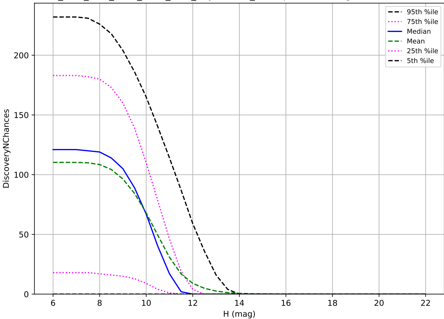
ddf_acor_sf20_lsf30_lsr50_v3.4_10yrs: OCC_r20 3 pairs in 15 nights detection loss
