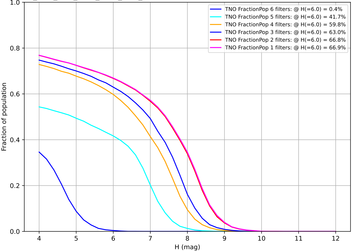
ddf_acor_sf20_lsf30_lsr50_v3.4_10yrs: Fraction of population with colors in X filters TNO
