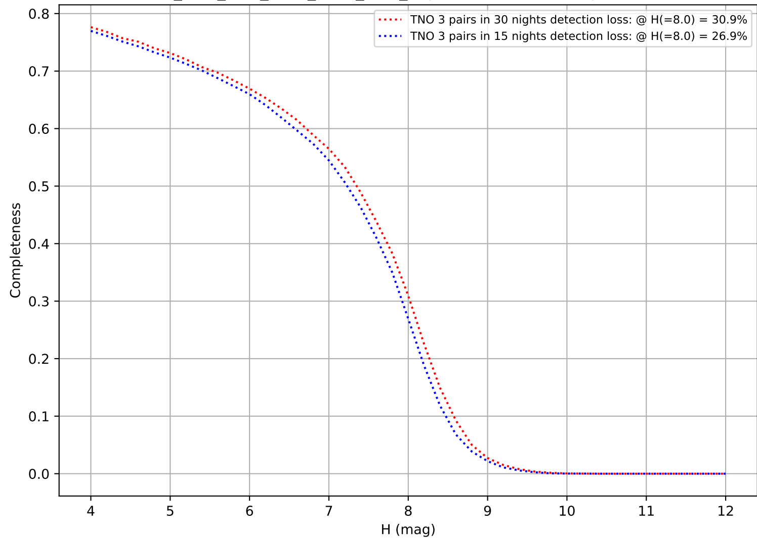
ddf_acor_sf20_lsf30_lsr50_v3.4_10yrs: DifferentialCompleteness
