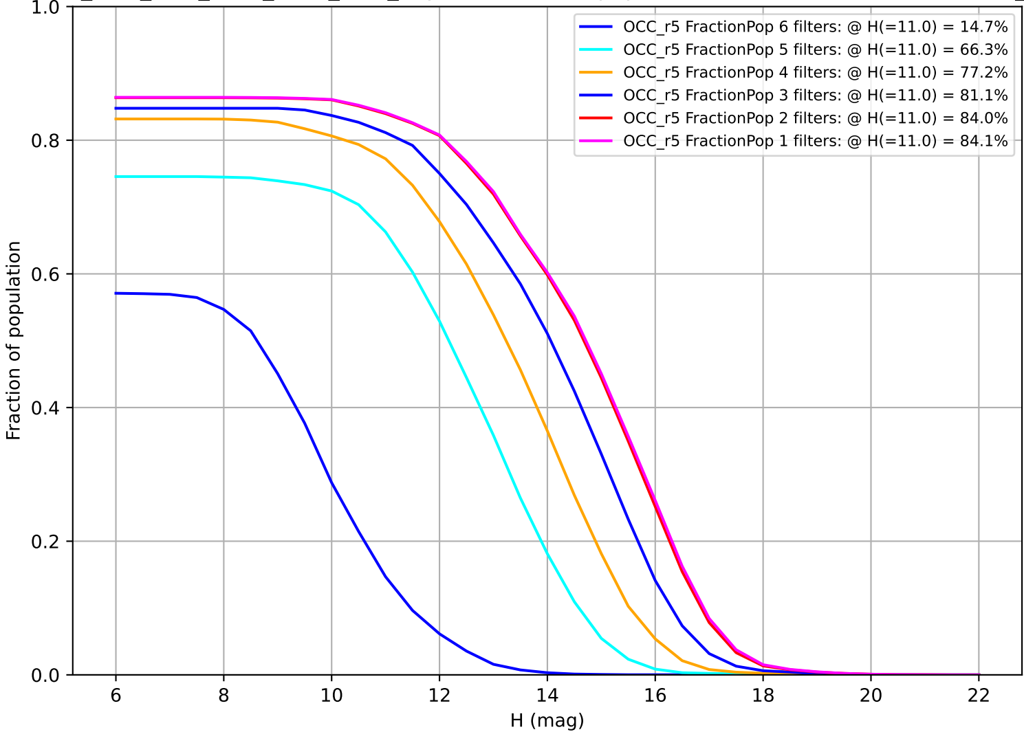
ddf_acor_sf20_lsf30_lsr50_v3.4_10yrs: Fraction of population with colors in X filters OCC_r5
