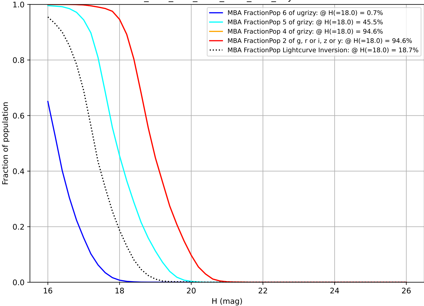
ddf_acor_sf20_lsf30_lsr50_v3.4_10yrs MBA
