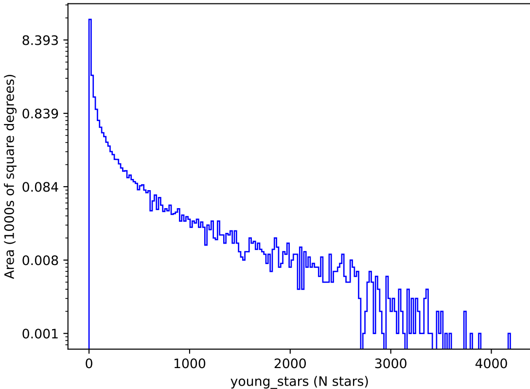
ddf_acor_sf20_lsf30_lsr50_v3.4_10yrs : young_stars
