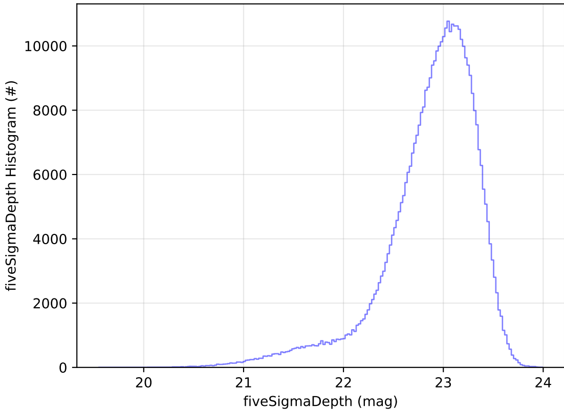
ddf_acor_sf20_lsf30_lsr50_v3.4_10yrs z: fiveSigmaDepth Histogram
