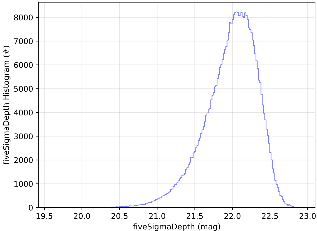
ddf_acor_sf20_lsf30_lsr50_v3.4_10yrs y: fiveSigmaDepth Histogram
