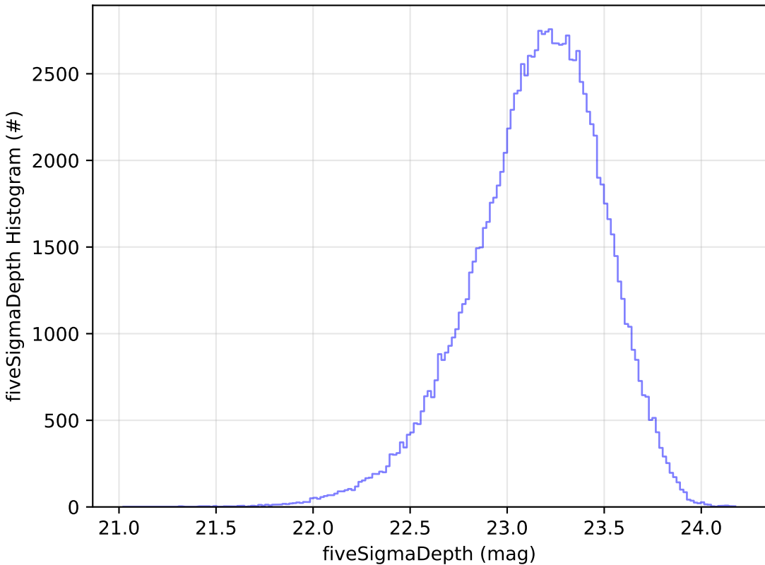
ddf_acor_sf20_lsf30_lsr50_v3.4_10yrs u: fiveSigmaDepth Histogram
