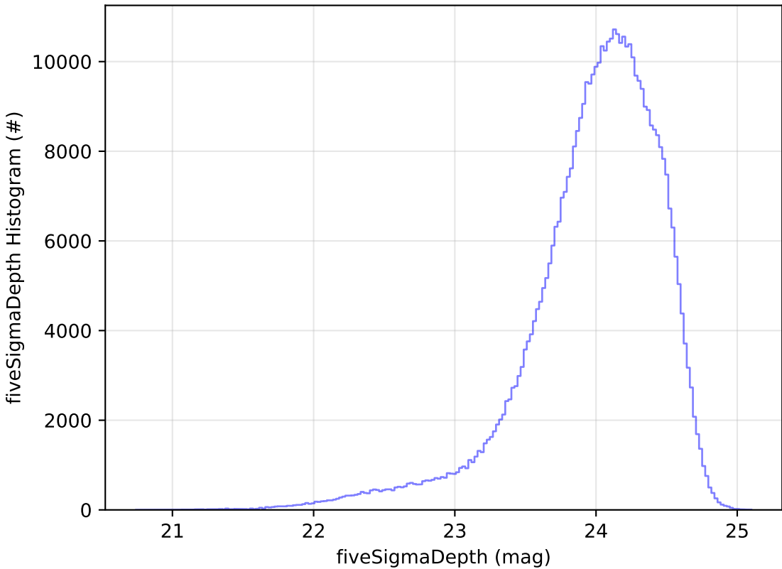
ddf_acor_sf20_lsf30_lsr50_v3.4_10yrs r: fiveSigmaDepth Histogram
