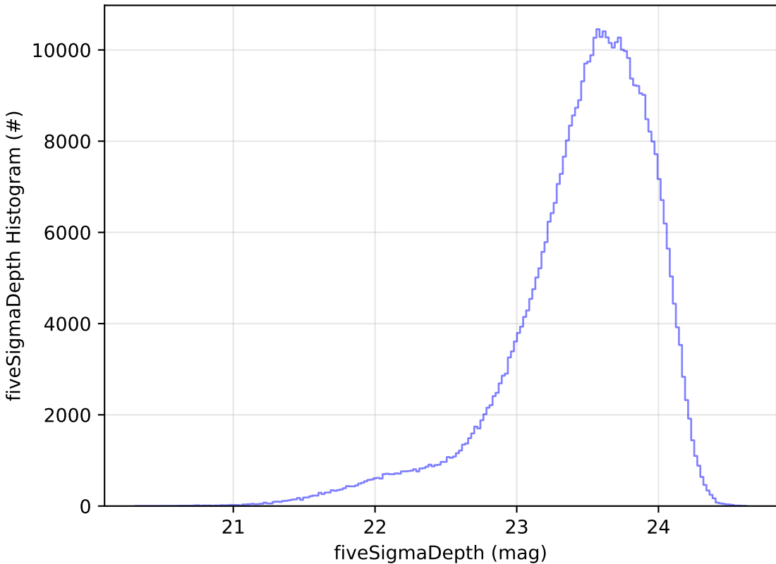
ddf_acor_sf20_lsf30_lsr50_v3.4_10yrs i: fiveSigmaDepth Histogram
