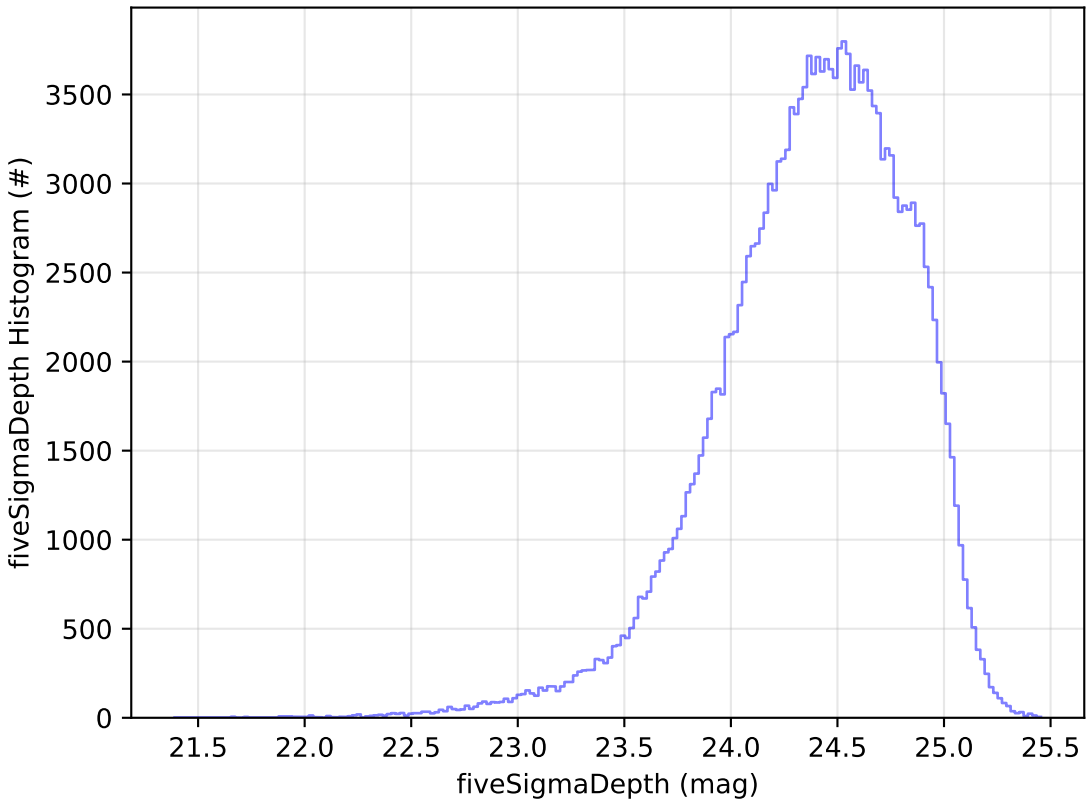
ddf_acor_sf20_lsf30_lsr50_v3.4_10yrs g: fiveSigmaDepth Histogram
