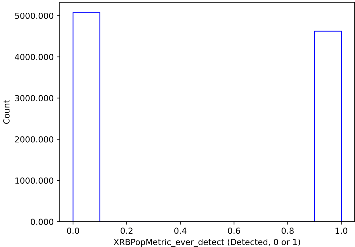
ddf_acor_sf20_lsf30_lsr50_v3.4_10yrs : XRBPoMetric_ever_detect
