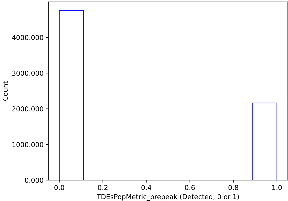
ddf_acor_sf20_lsf30_lsr50_v3.4_10yrs : TDEsPopMetric_prepeak
