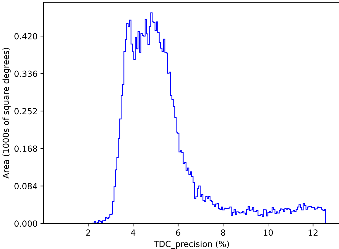
ddf_acor_sf20_lsf30_lsr50_v3.4_10yrs : TDC_precision
