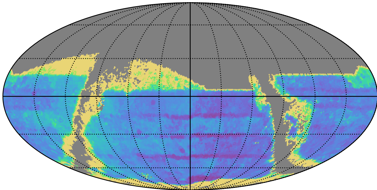
ddf_acor_sf20_lsf30_lsr50_v3.4_10yrs : TDC_accuracy
