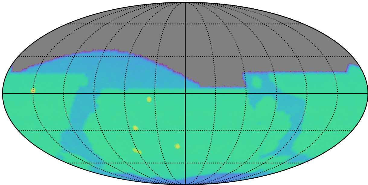
ddf_acor_sf20_lsf30_lsr50_v3.4_10yrs i: SurfaceBrightLimit
