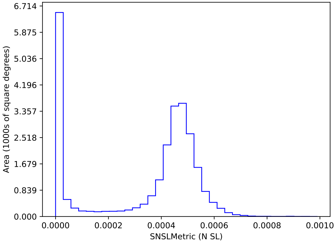
ddf_acor_sf20_lsf30_lsr50_v3.4_10yrs : SNSLMetric
