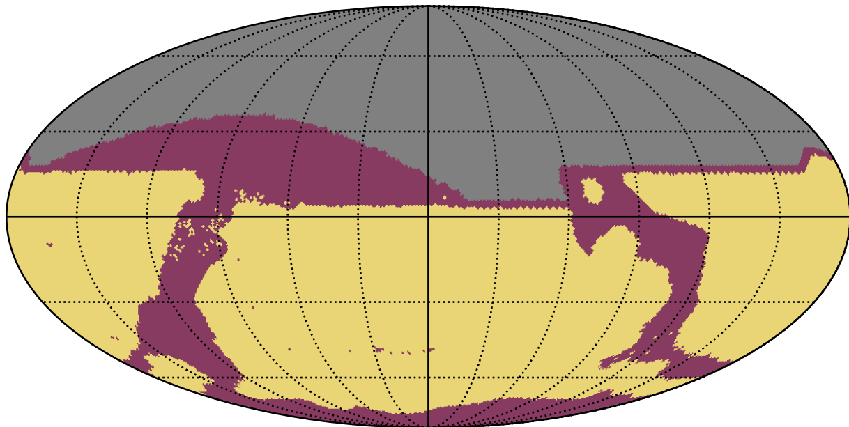
ddf_acor_sf20_lsf30_lsr50_v3.4_10yrs : RapidRevisits
