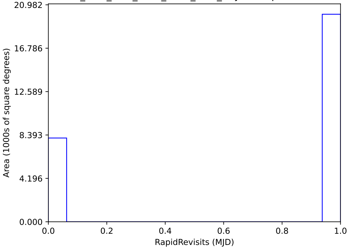
ddf_acor_sf20_lsf30_lsr50_v3.4_10yrs : RapidRevisits
