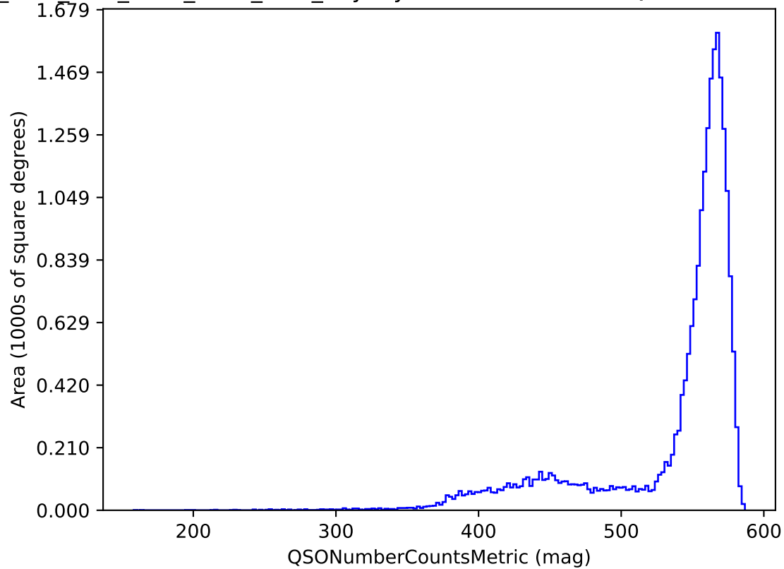
ddf_acor_sf20_lsf30_lsr50_v3.4_10yrs y band and non-DD: QSONumberCountsMetric
