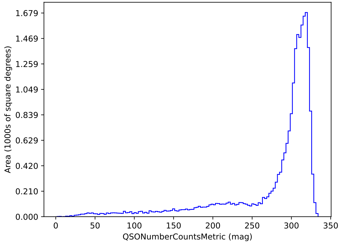
ddf_acor_sf20_lsf30_lsr50_v3.4_10yrs u band and non-DD: QSONumberCountsMetric
