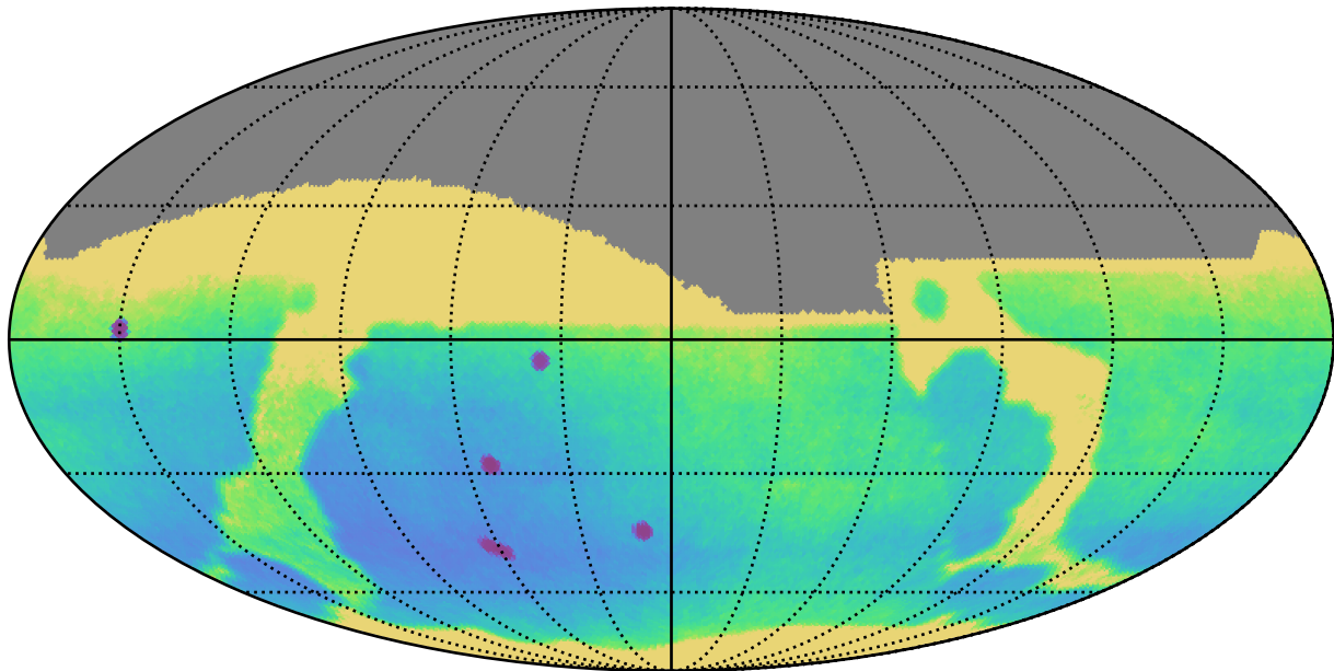
ddf_acor_sf20_lsf30_lsr50_v3.4_10yrs : Parallax Uncert @ 24.0
