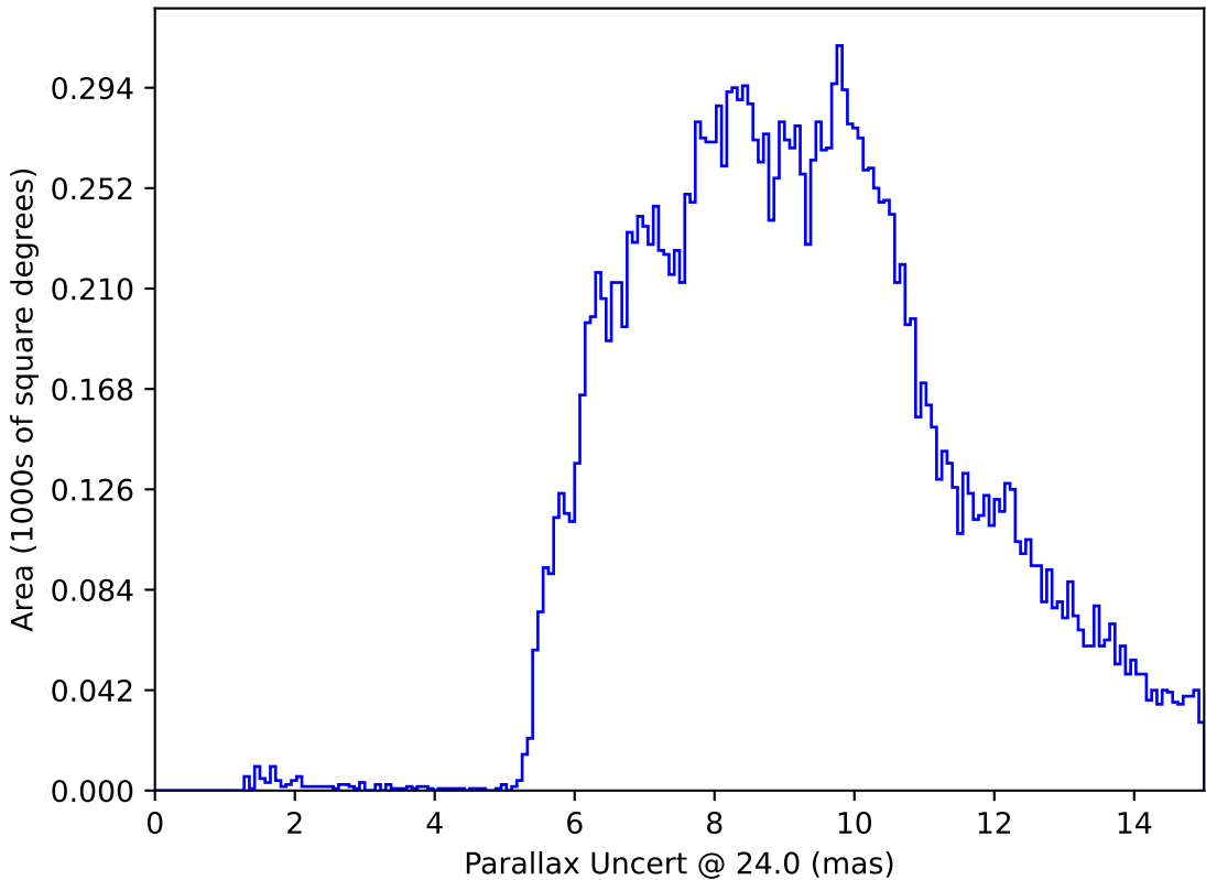
ddf_acor_sf20_lsf30_lsr50_v3.4_10yrs : Parallax Uncert @ 24.0
