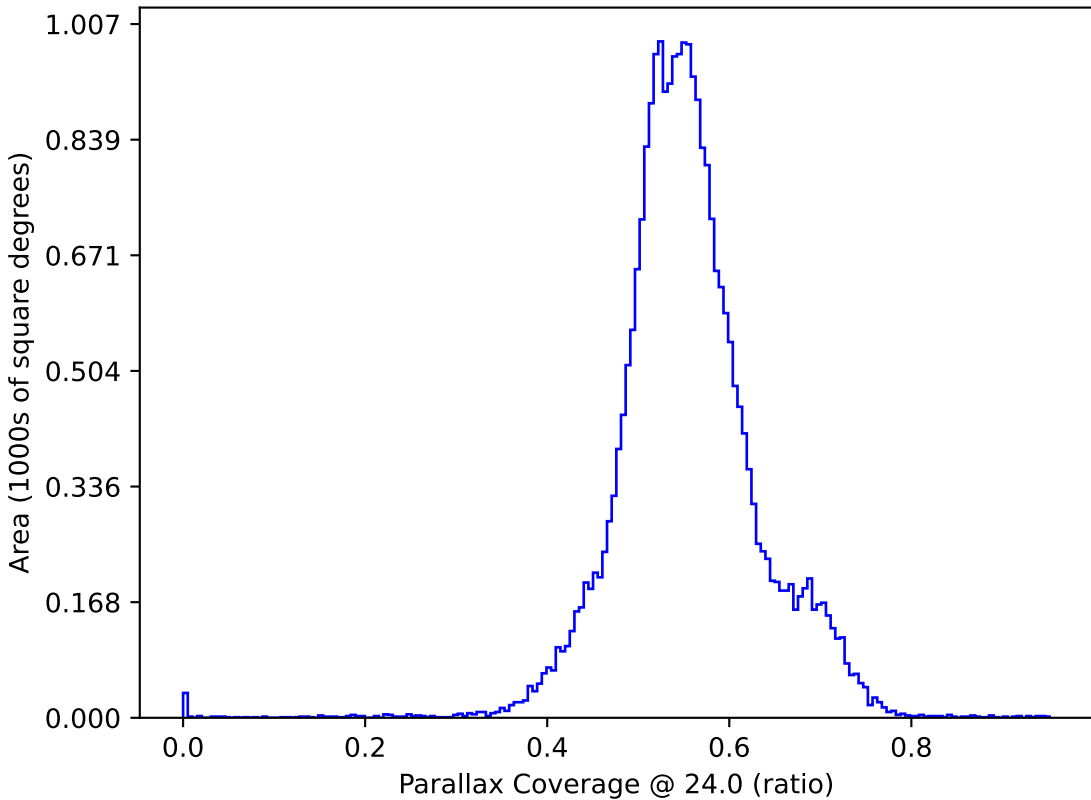
ddf_acor_sf20_lsf30_lsr50_v3.4_10yrs : Parallax Coverage @ 24.0
