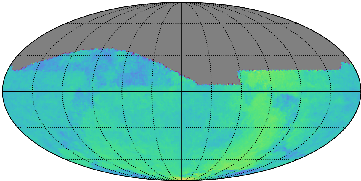
ddf_acor_sf20_lsf30_lsr50_v3.4_10yrs : Parallax Coverage @ 22.4
