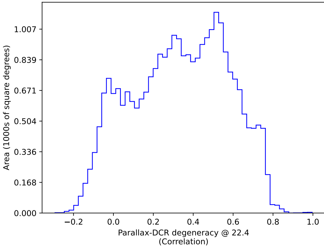
ddf_acor_sf20_lsf30_lsr50_v3.4_10yrs : Parallax-DCR degeneracy @ 22.4
