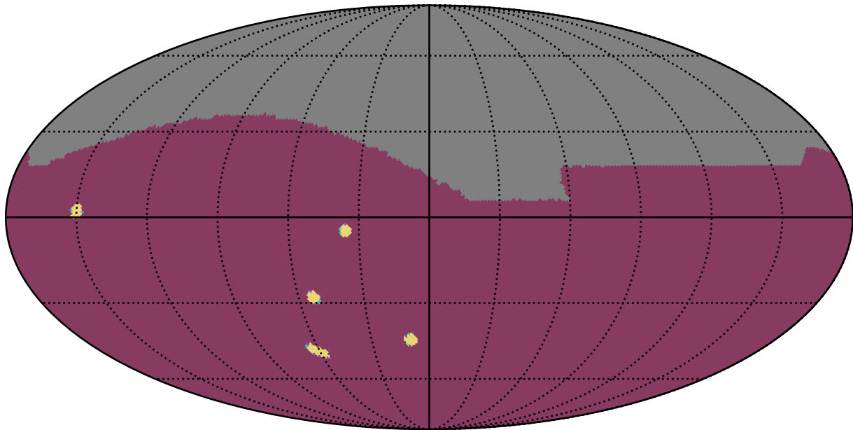
ddf_acor_sf20_lsf30_lsr50_v3.4_10yrs : NumberOfQuickRevisits
