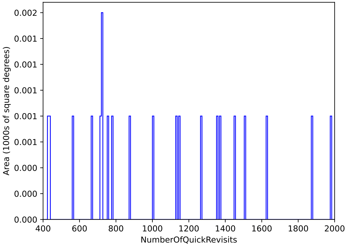
ddf_acor_sf20_lsf30_lsr50_v3.4_10yrs : NumberOfQuickRevisits
