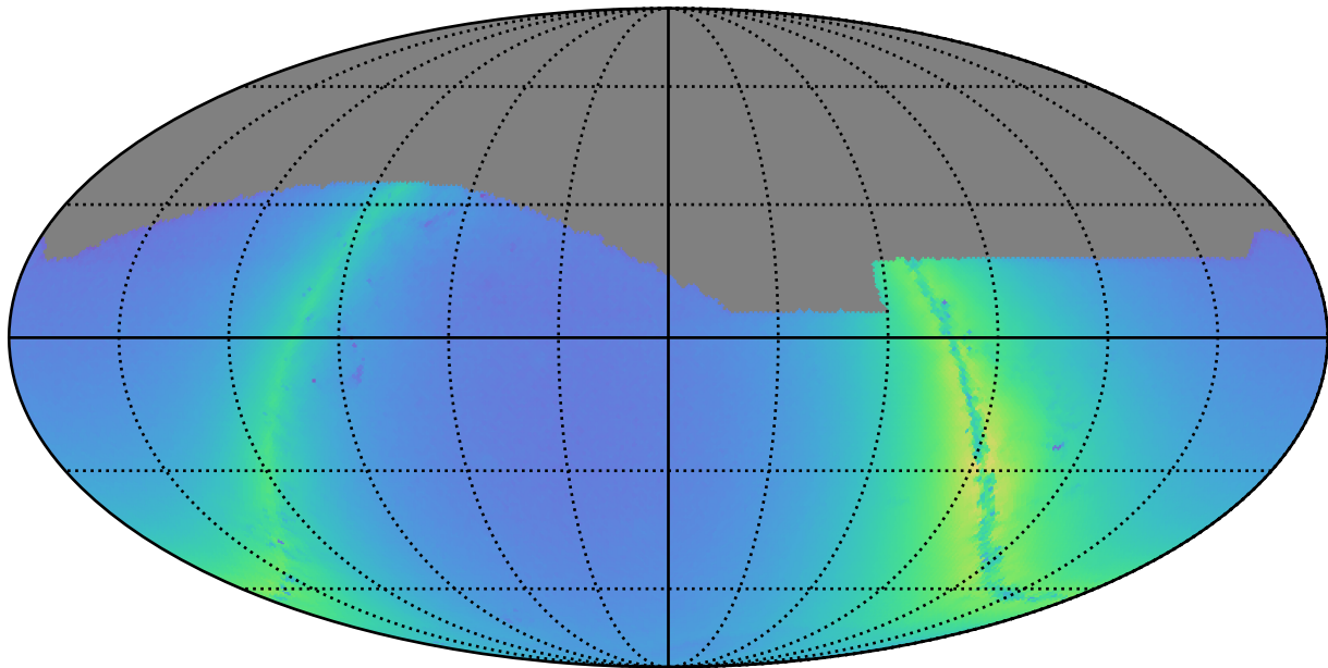
ddf_acor_sf20_lsf30_lsr50_v3.4_10yrs r: Nstars_no_crowding
