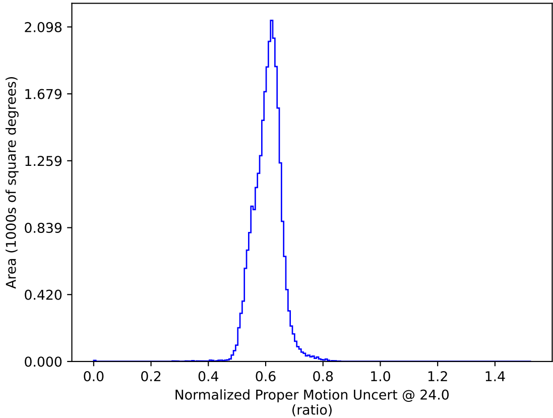
ddf_acor_sf20_lsf30_lsr50_v3.4_10yrs : Normalized Proper Motion Uncert @ 24.0
