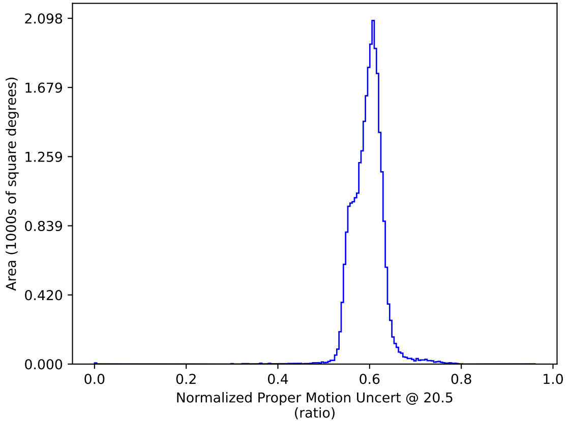
ddf_acor_sf20_lsf30_lsr50_v3.4_10yrs : Normalized Proper Motion Uncert @ 20.5
