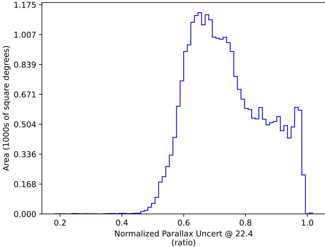
ddf_acor_sf20_lsf30_lsr50_v3.4_10yrs : Normalized Parallax Uncert @ 22.4
