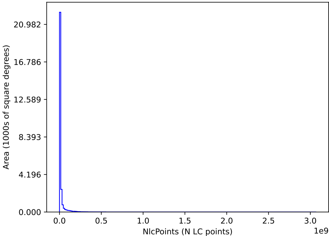
ddf_acor_sf20_lsf30_lsr50_v3.4_10yrs : NlcPoints
