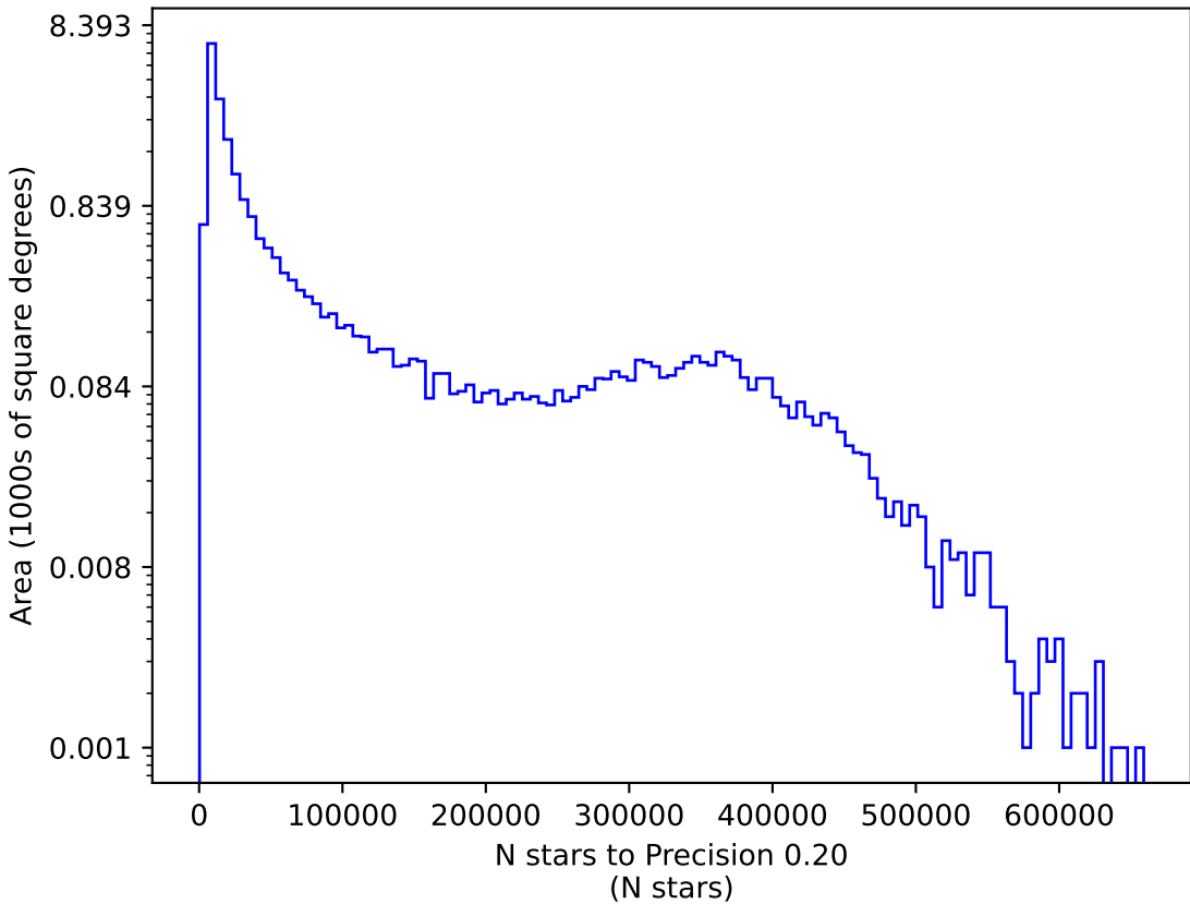
ddf_acor_sf20_lsf30_lsr50_v3.4_10yrs y: N stars to Precision 0.20
