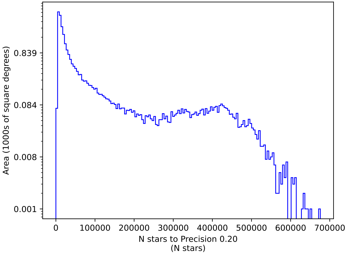
ddf_acor_sf20_lsf30_lsr50_v3.4_10yrs r: N stars to Precision 0.20
